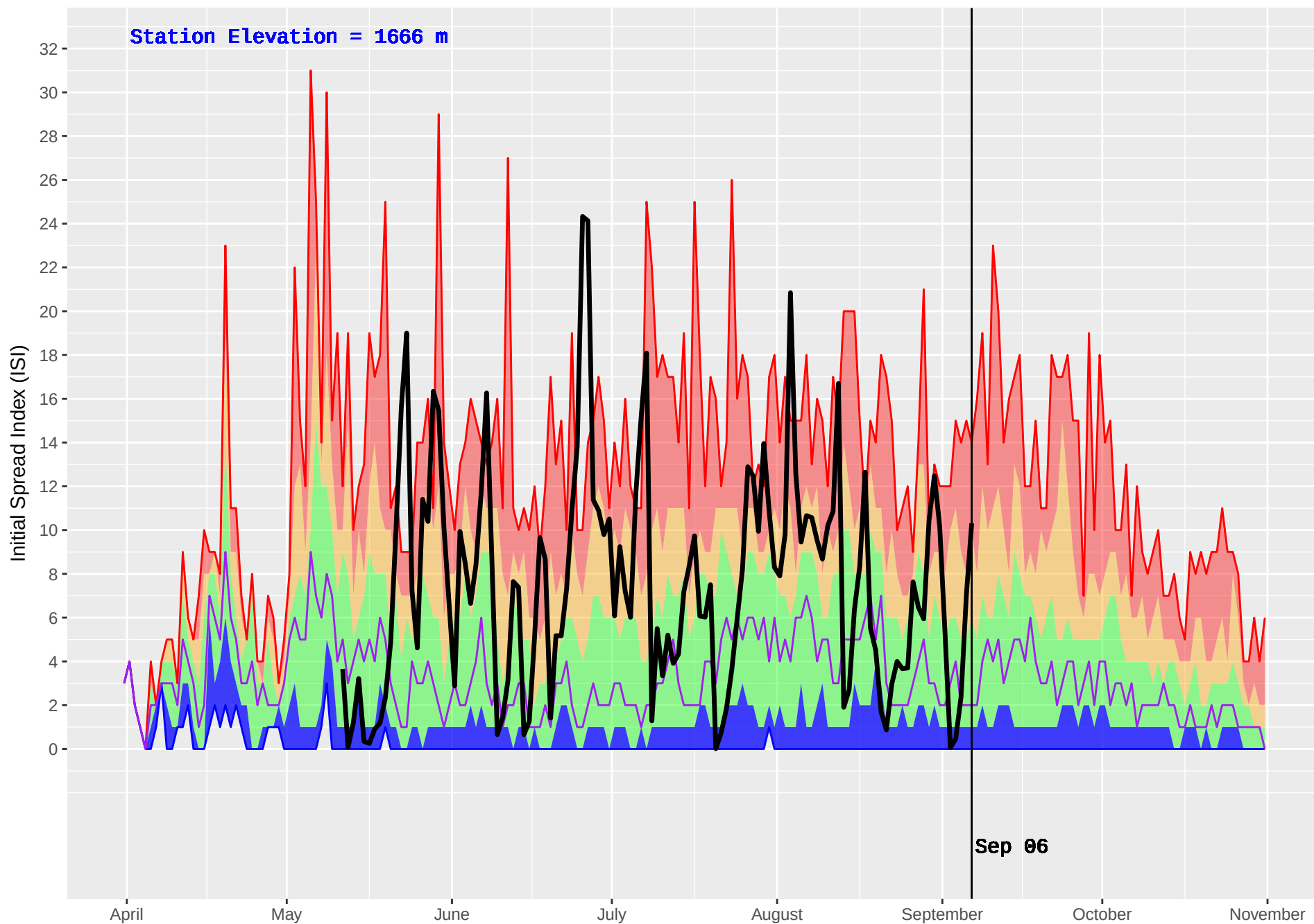
BALDFACE (221) : Historical (1992–2016) and Current (2017) Noon Initial Spread Index (ISI)
